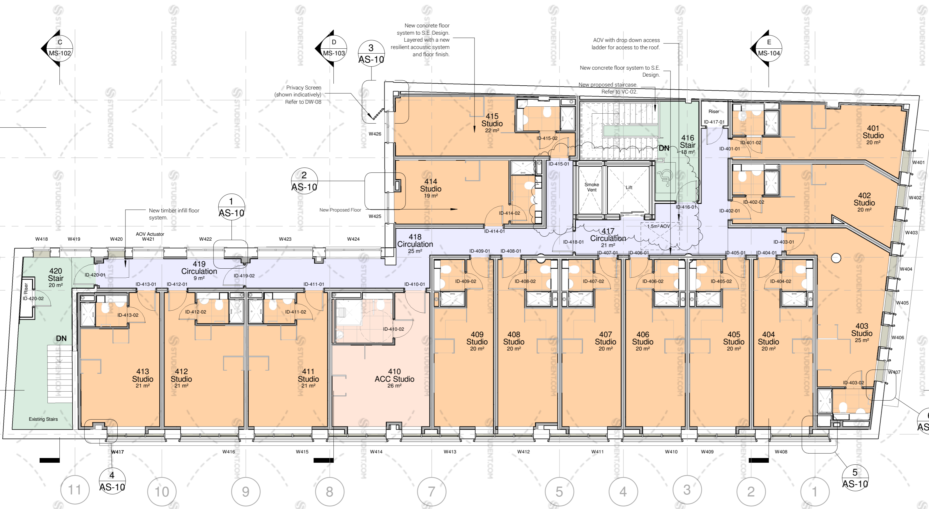
Proposed Fourth Floor Plan 1 : 100
